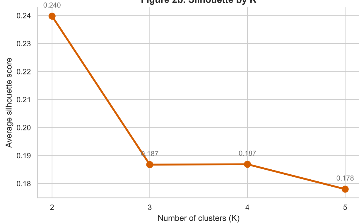
Figure 2b. Silhouette by K
