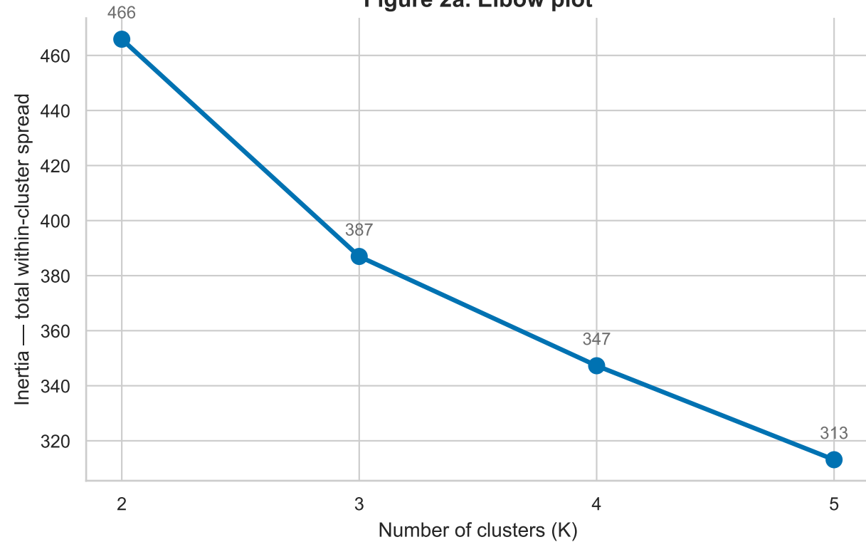
Figure 2a. Elbow plot
